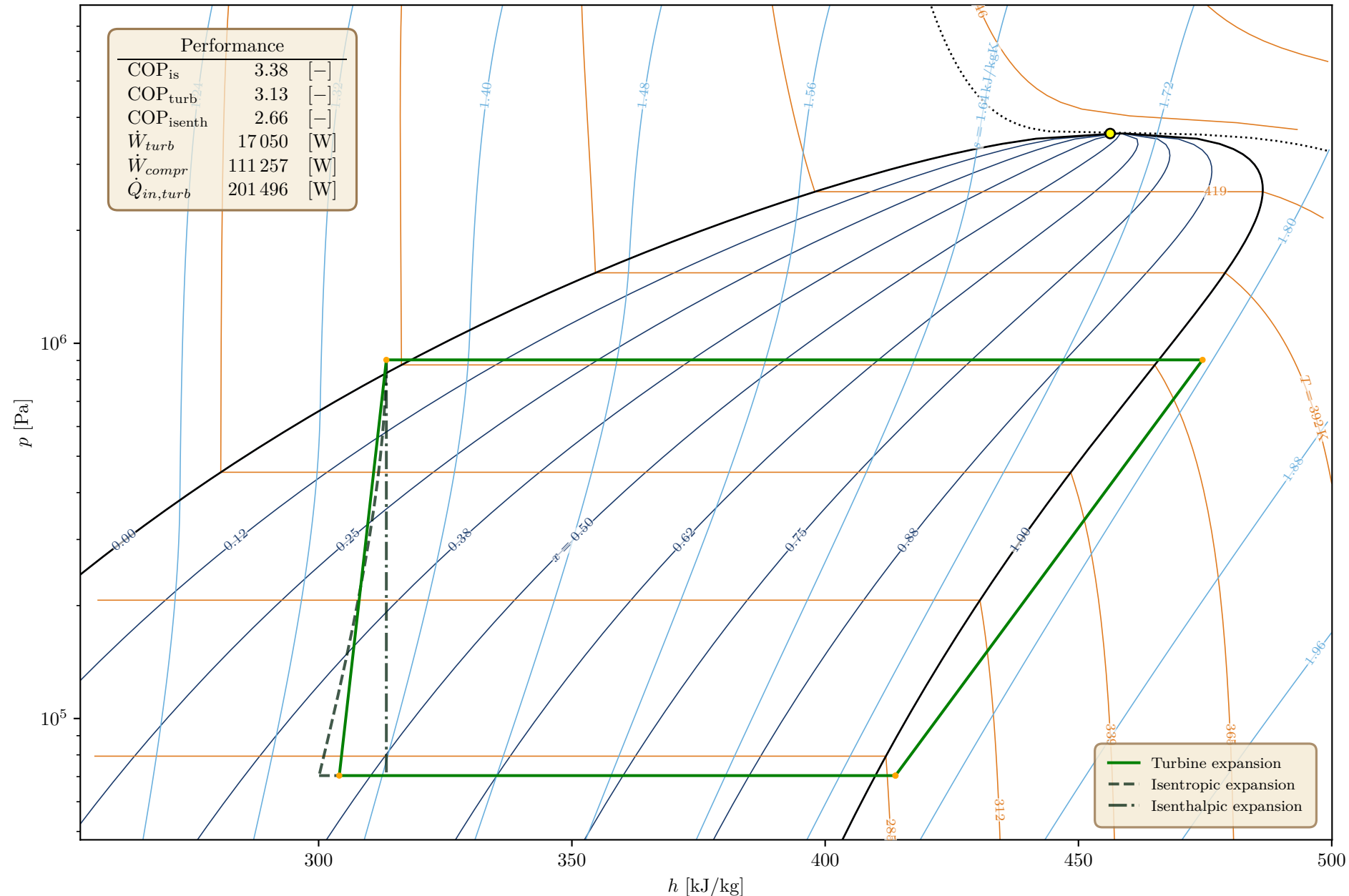
Conceptual Heat Pump Cycle – R1233zd(E)
